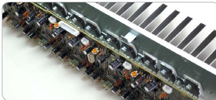
Fully discrete power amplifiers for all 5 channels
